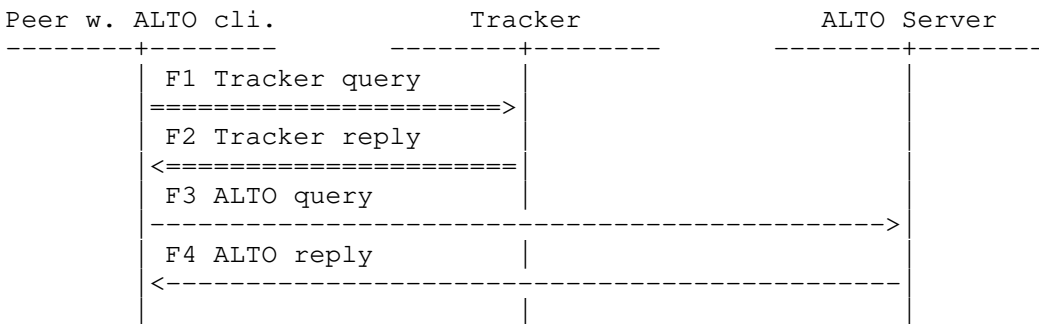
Figure 1: Tracker-Based P2P Application with Random Peer Preselection
